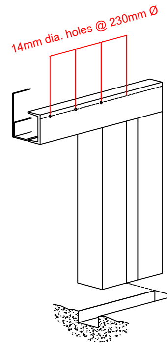
R.S. CHANNEL LINTEL
