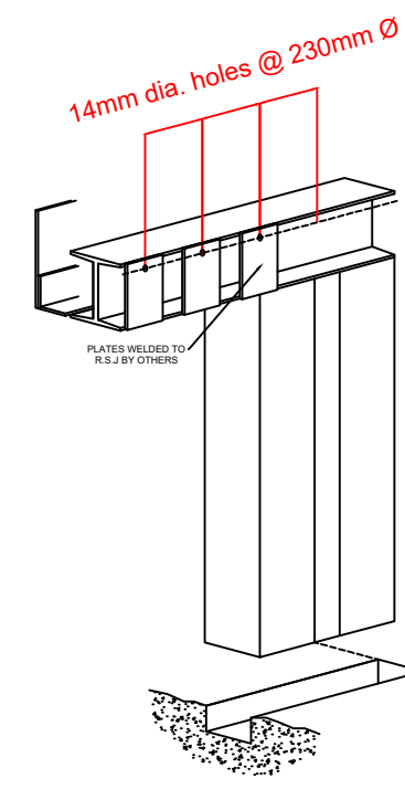
R.S. JOIST LINTEL
