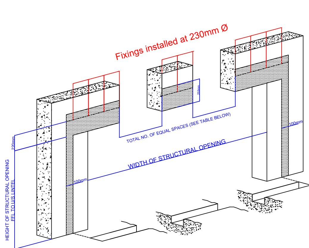
ELEVATION VIEWED FROM INSIDE
